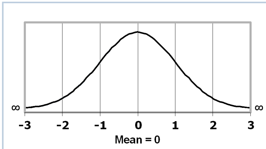
FIGURE 3 Normal Distribution
